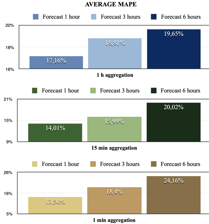
Fig. 7. Average MAPE at different time horizons and time aggregations (ARIMA)
