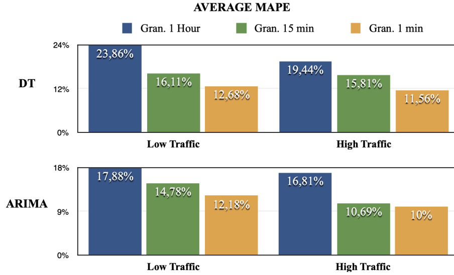
Fig. 6. Average 1 Step MAPE details for the two traffic levels
