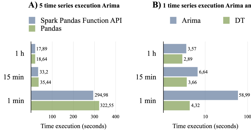
Fig. 8. Execution time comparisons
