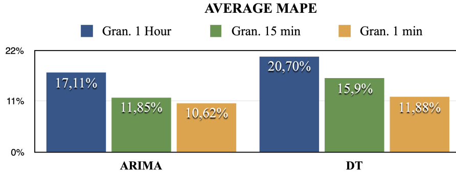
Fig. 4. Average 1 Step MAPE for the two models at different data granularities
