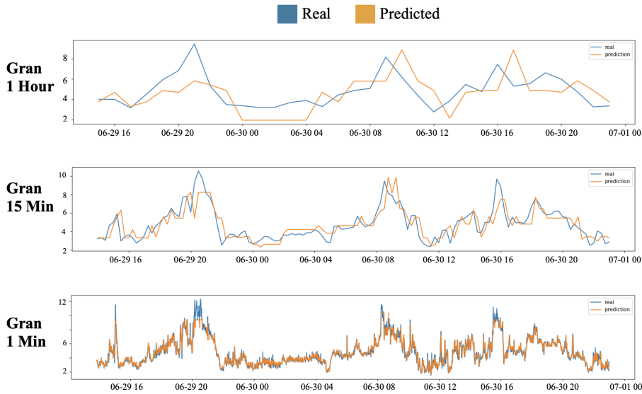
Fig. 5. 1 Step forecast for a single time series in relation to different time granularities
